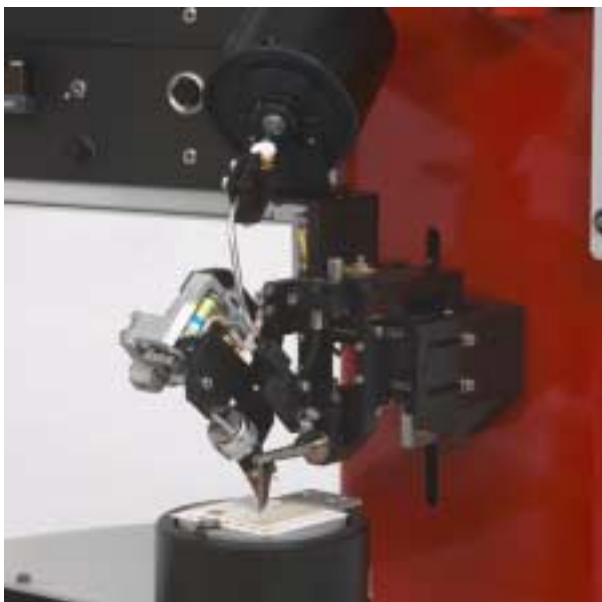
Bondhead 5330 4.2034.2000 new designed mechanical clamp (Feed&Tail)
