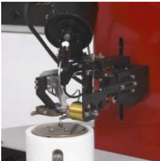
Bondhead 5310 4.2034.1000 with Flame-Off
