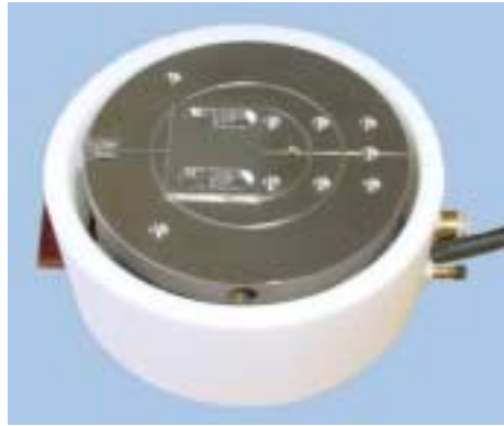
Option TB0000.87.000 heated Ø 80mm, mechanical clamping and vacuum
